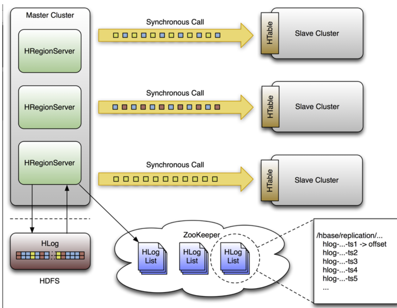
Figure 18. Replication Architecture Overview
